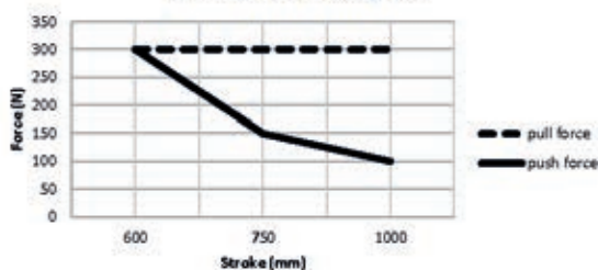
Stroke/force diagram
